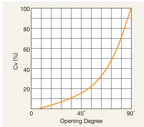
Valve Opening vs. Cv
